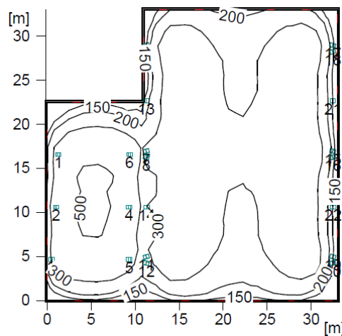
(既存メタハラ1000W)
